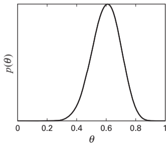
Beta(15,10)
