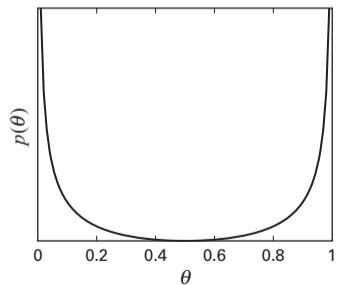
Beta(0.5,0.5)
