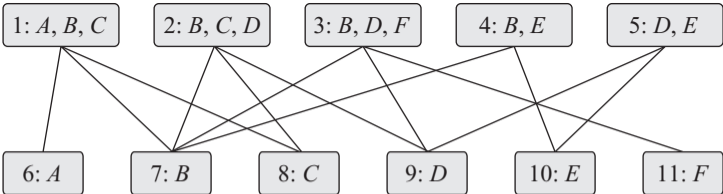
(a) \mathcal{U}_3
