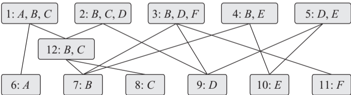
(b) \mathcal{U}_4
